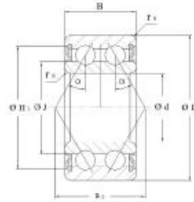
32...2RS , 33...2RS , 38...2RS
