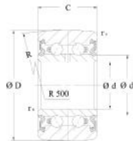
LR 50..NPPU, LR 52..NPPU, LR 53..NPPU
