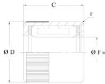
HF..R, HF..KFR with knurled outer ring
